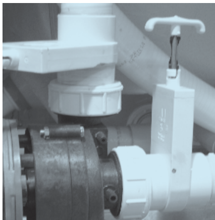
Slice Valve and Pump Union
